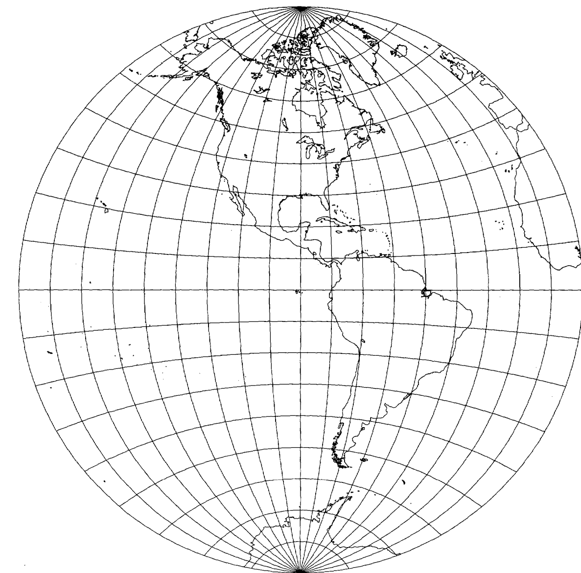
Figure 73.—Nicolosi Globular projection, with shorelines, 10° graticule. Central meridian 90° W.
