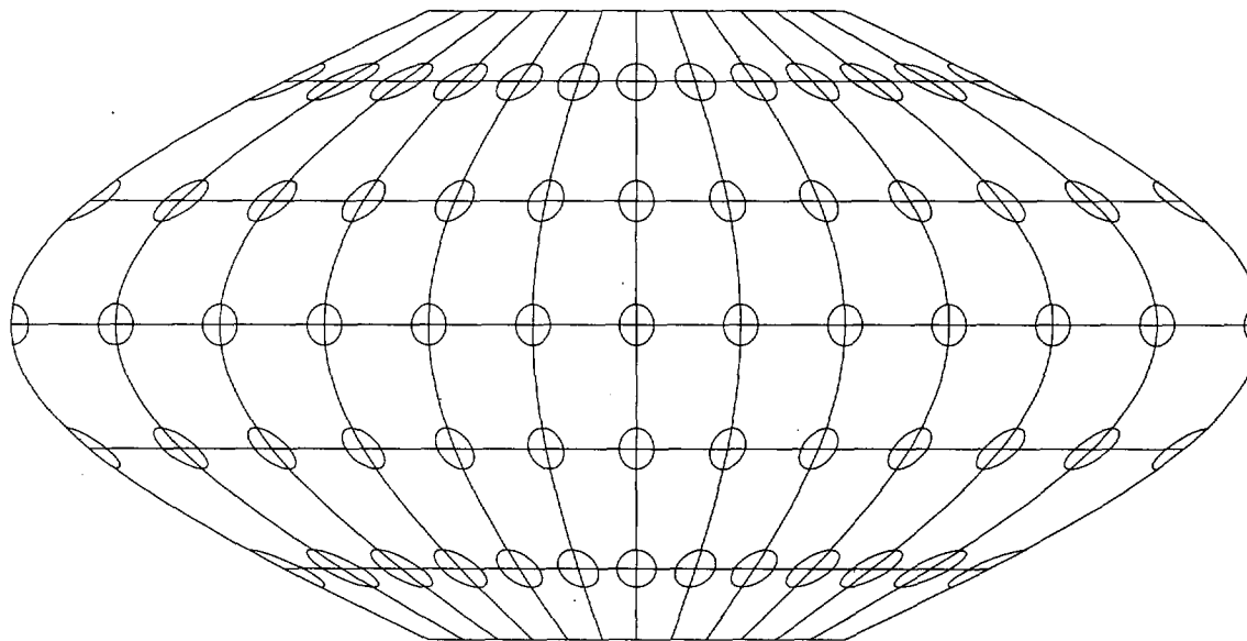
Figure 14A.—McBryde-Thomas Flat-Polar Sinusoidal projection, with Tissot indicatrices, 30^{\circ} graticule.
