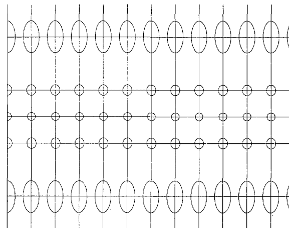
Figure 10A.—Central Cylindrical projection with Tissot indicatrices, 30° graticule.
