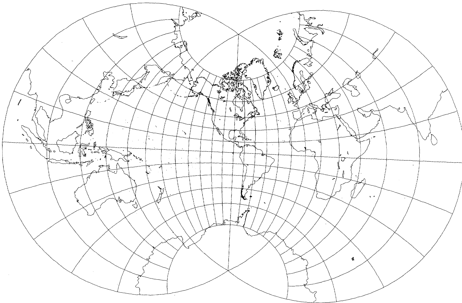
Figure 76C.—Lagrange projection of 0.7 of sphere in circle, with shorelines, 15° graticule. Central meridian 90° W.
