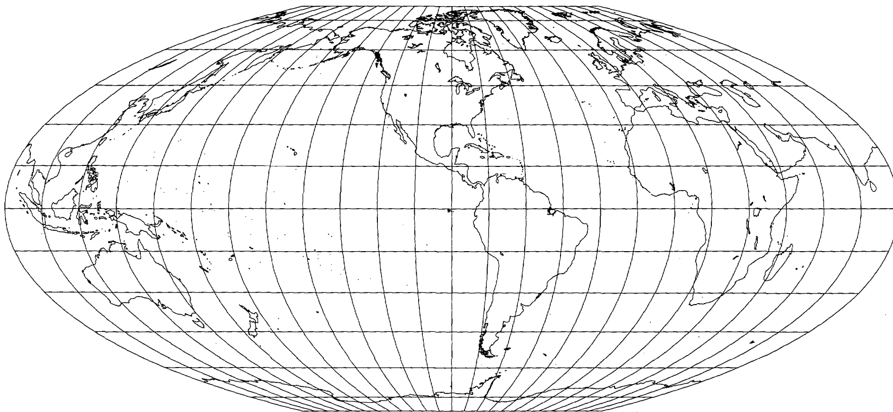
Figure 29B.—McBryde-Thomas Flat-Polar Quartic projection, with shorelines, 15° graticule. Central meridian 90° W.
