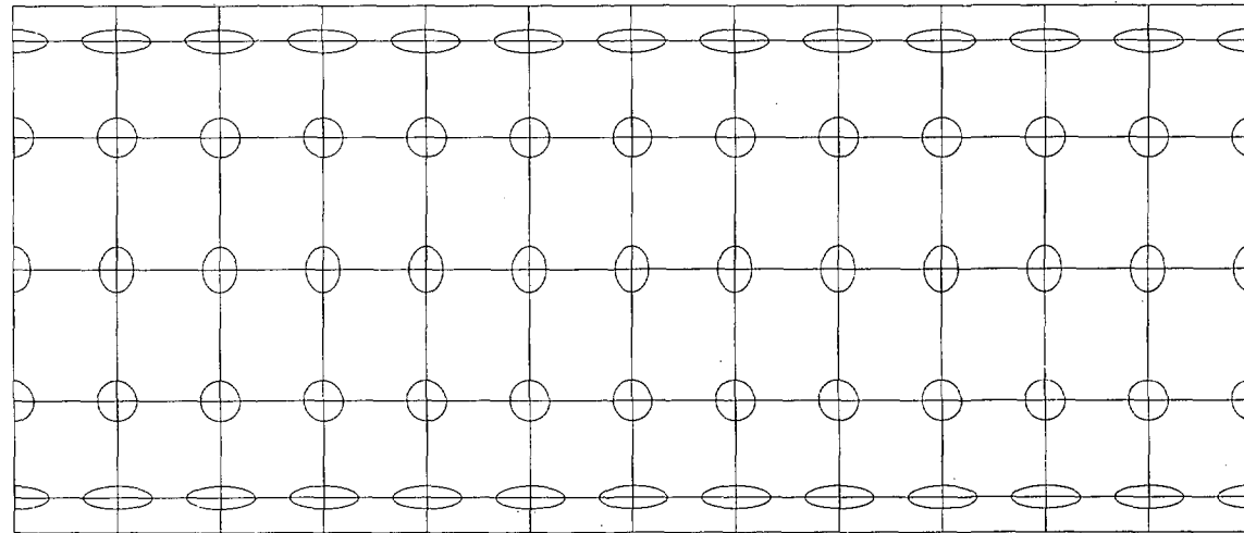
Figure 5A.—Behrmann Cylindrical Equal-Area projection with Tissot indicatrices, 30^\circ graticule. Standard parallels 30^\circ N. and S.
