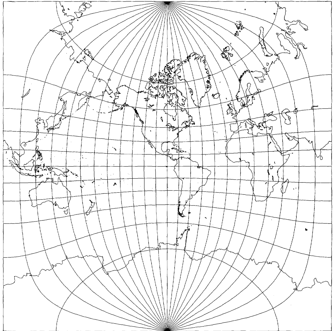
Figure 82.—Adams projection of the world in a square I, with shorelines, 15° graticule. Central meridian 90° W.
