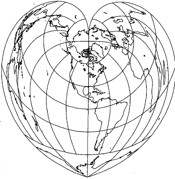
Figure 46C.—Werner projection, with shorelines, 30° graticule. Central meridian 90° W. Polar limit of Bonne projection.
