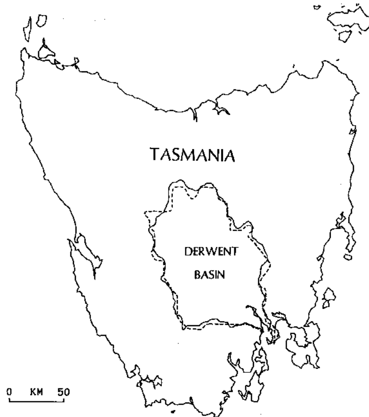
Fig 9. The Derwent River catchment of Tasmania, after Figure 2 of Hutchinson and Dowling (1991). The solid line denotes the boundary calculated from a 1/40th-degree DEM. The dashed line denotes the boundary calculated from a 1/20th-degree DEM.
